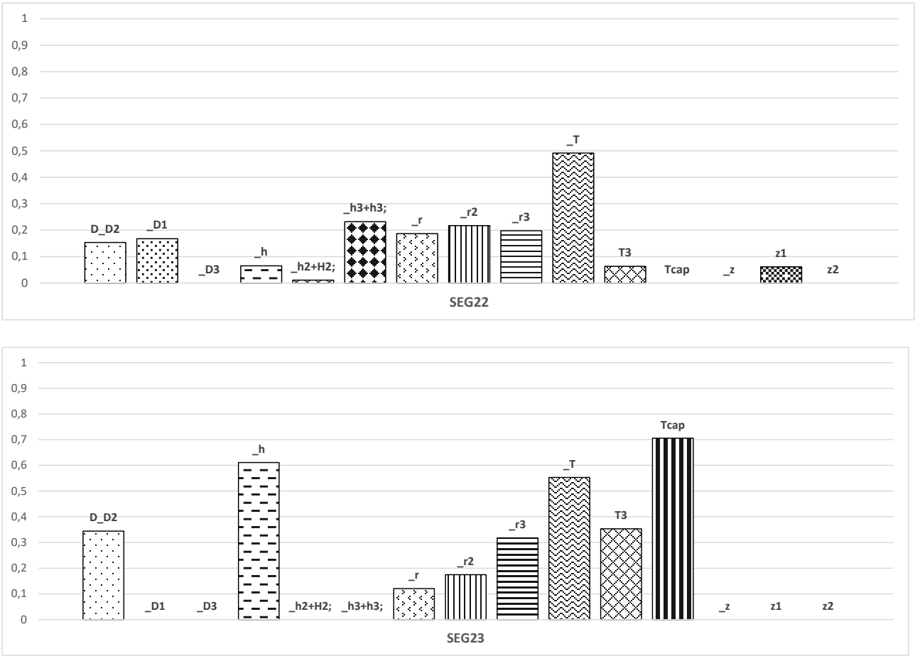
TAVOLA 34: Esempio di istogrammi a tre varianti (/D/+/&D2;/ vs /&D3;/ vs /&D1;/; /h/ vs /&h3;/+/&h3/ vs /&h2;/+/&h2;/ /r/ vs /&r3;/ vs /&r2;/; /T/ vs /&T3;/ vs /&Tcap;/; /z/ vs /&z1;/ vs, /&z2;/) per i segmenti 22 e 23
